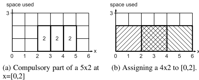
Figure 2: Examples of compulsory parts and intervals.
