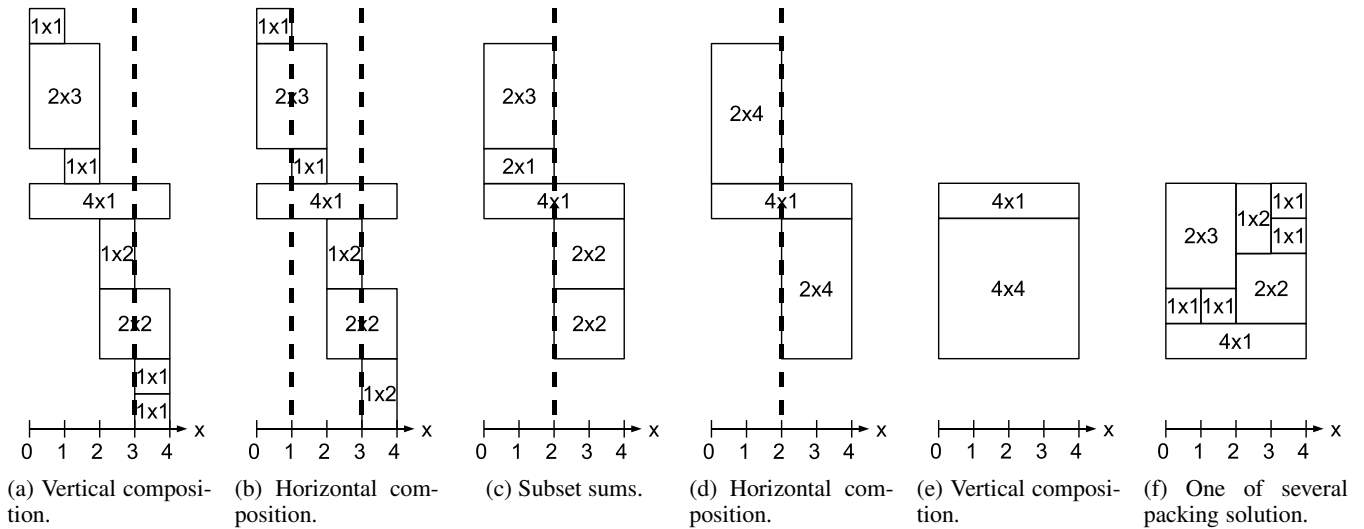
Figure 3: Examples of composing rectangles and subset sums.
